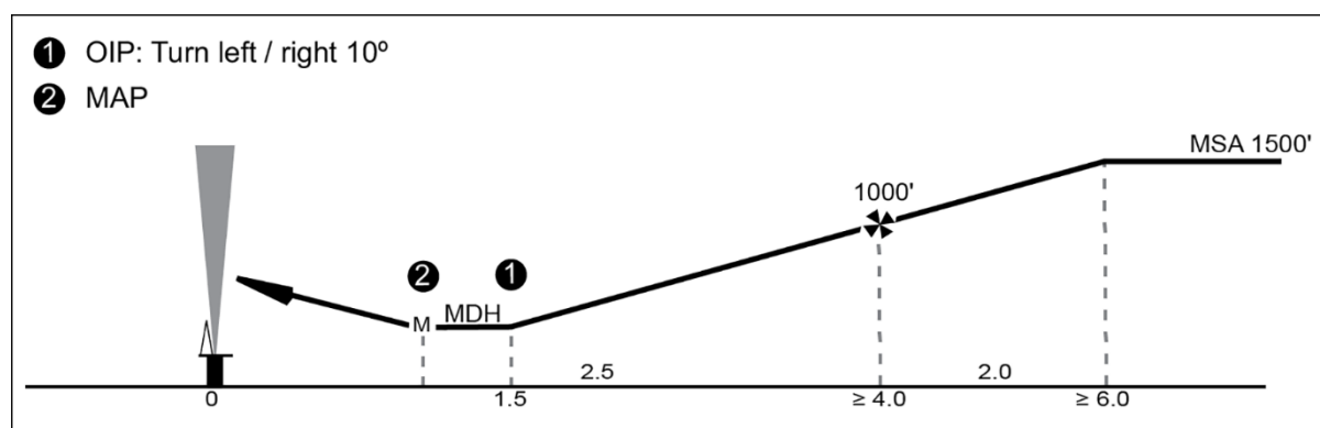
Figure 2 — Vertical profile
