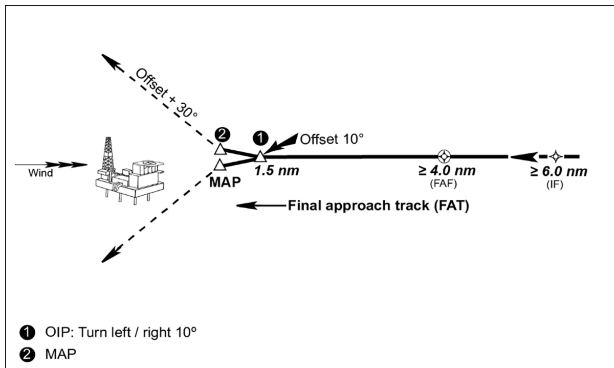
Figure 1 — Horizontal profile
